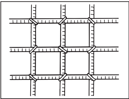
③ Tie in alternate direction.
