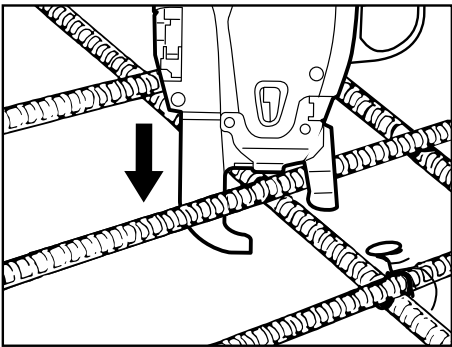
② Apply the tool perpendicularly to the surface of the crossed re-bars.
