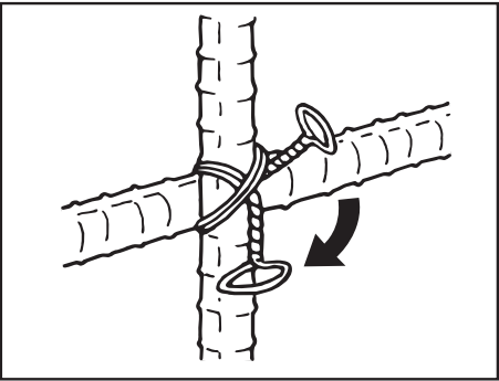
④ Cross tie. Bent the tail of the first tie before making the second tie.
