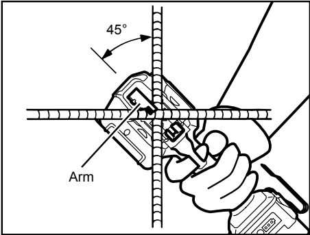
① Tilt the tool 45° angle to the crossed re-bars.
