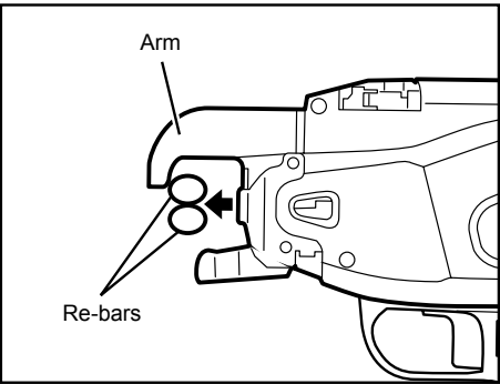
⑤ When you need extra tightness, place re-bars at the top of the Arm part.
